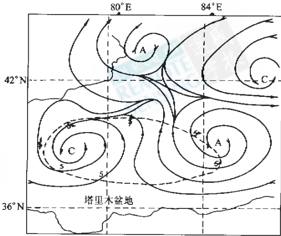
图4 1999-04-24 14时的天气图(→流线----能见度<1 km区) Fig. 4 Weather map at 12:00 UTC on April 24th, 1999
