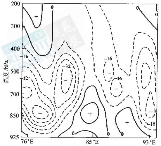
图6 1999-04-24 20时的沿38°N垂直速度剖面图 Fig. 6 ( \omega ) cross-section diagram (along 38°N) at 12:00 UTC on April 24th, 1999
